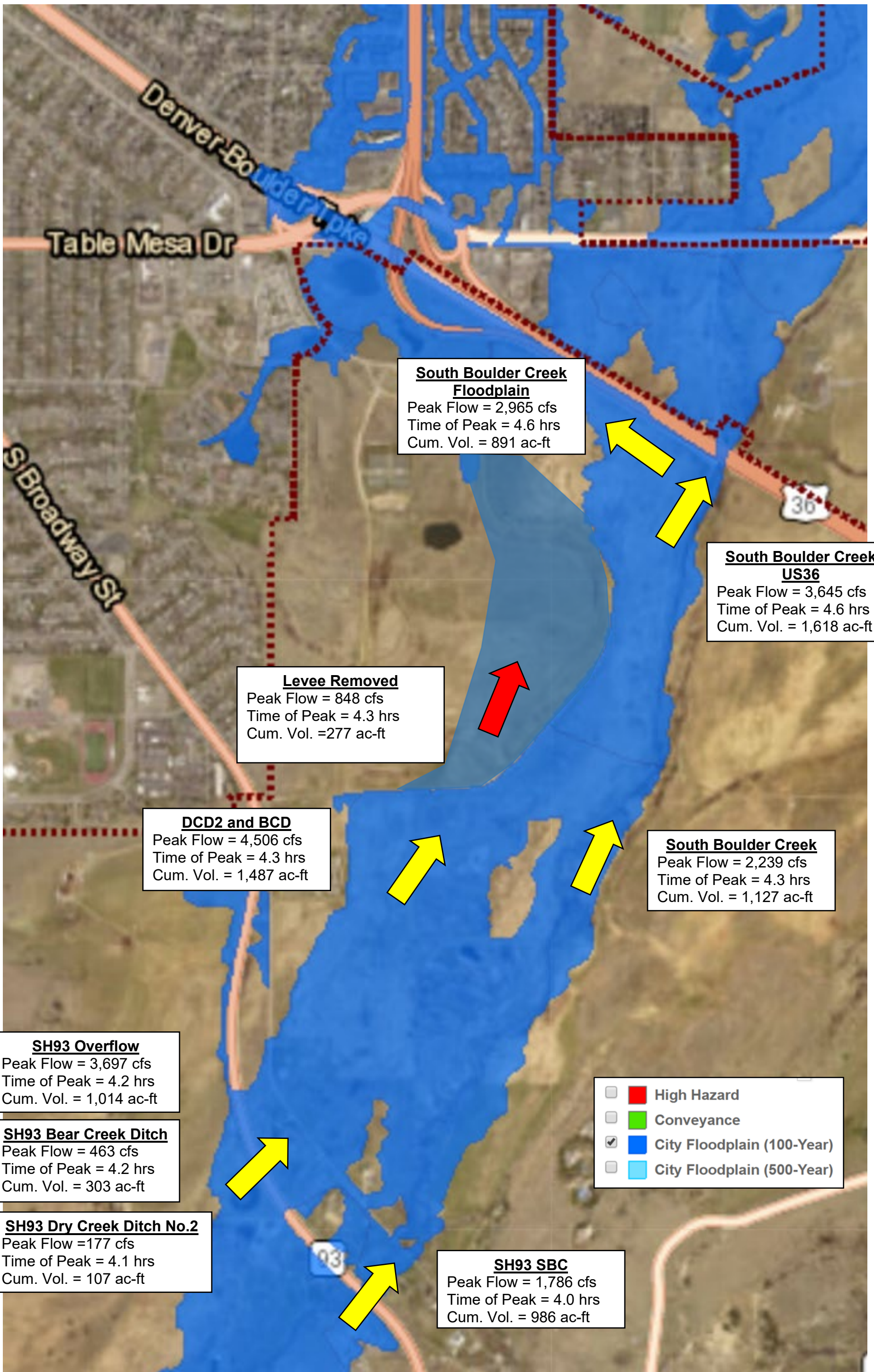
South Boulder Creek 100-yr Flood Flows – Levee Removed
