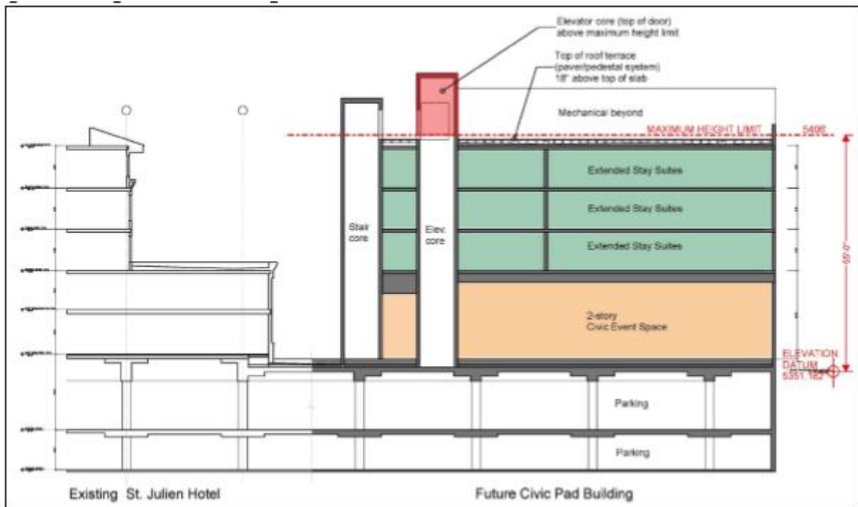
Figure 2 – Diagrammatic Building Section
