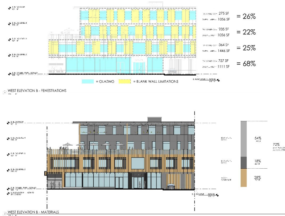
Figure 1: Example of fenestration pattern per floor, and percentage and type of materials
